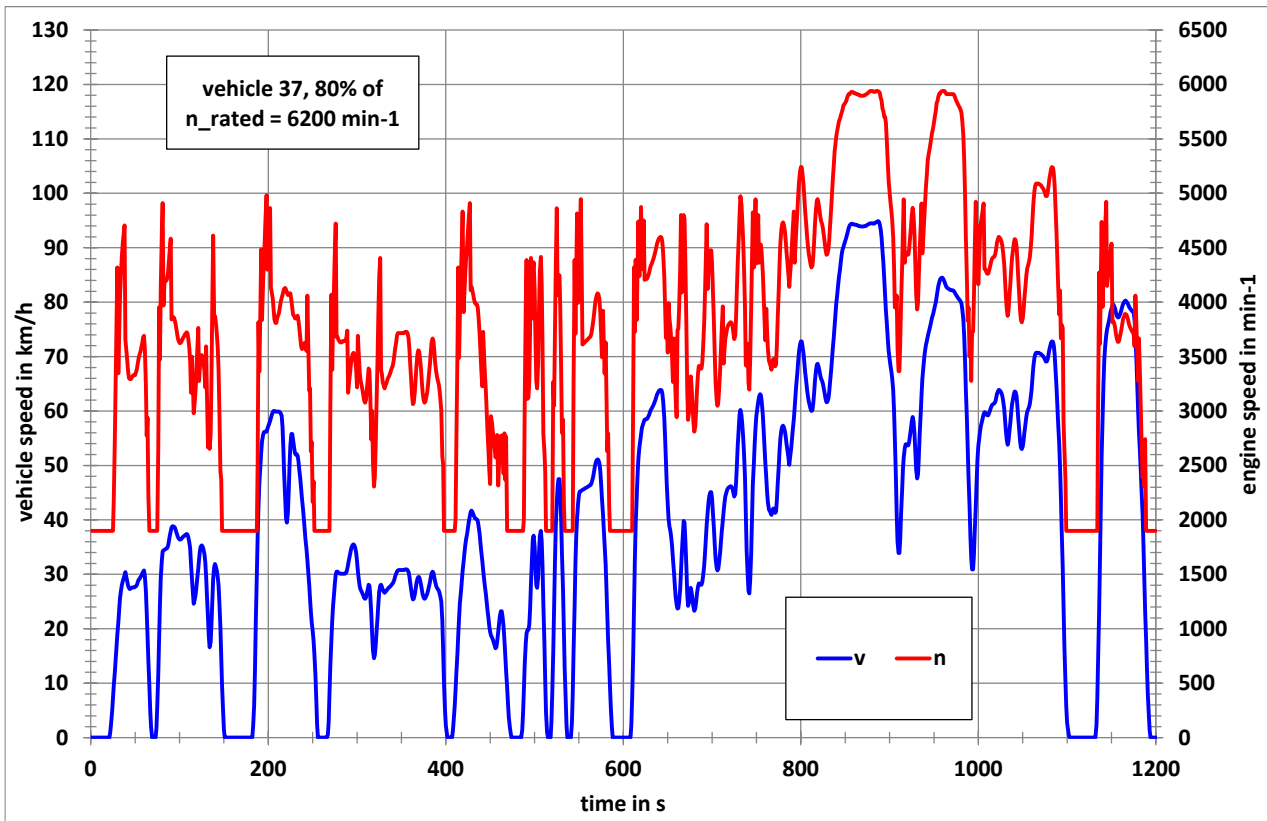
Figure 3-7: Vehicle speed and engine speed time series of the WMTC cycle for vehicle 37 of the EU WMTC in use database
