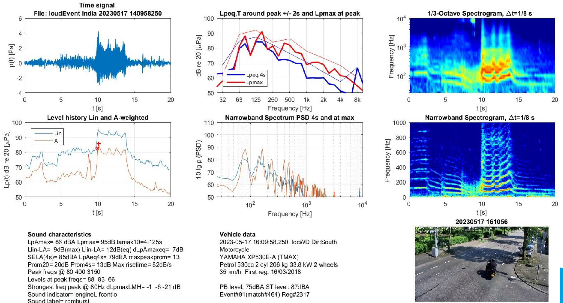
Figure B-13: Sound characteristics of a motorcycle, example of 'rpmburst'
