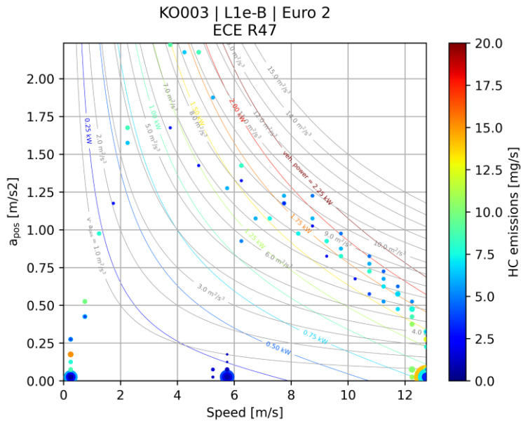
Figure C-8: HC emission map (cold phase)
