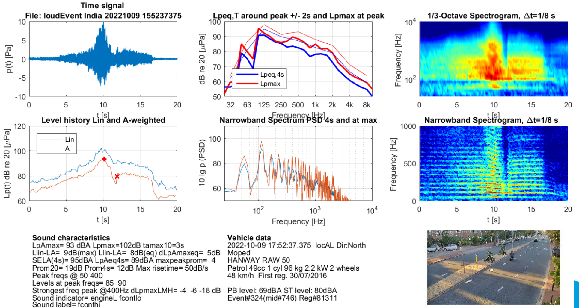
Figure B-11: Sound characteristics of a moped, example of 'fconthi/rpmconthi'
