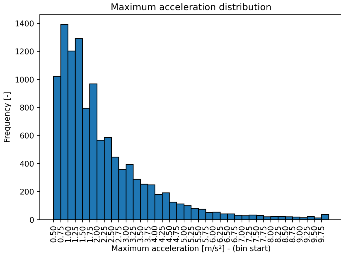
Figure 2-31: Maximum acceleration distribution for radar measurements at the first two locations in Utrecht
