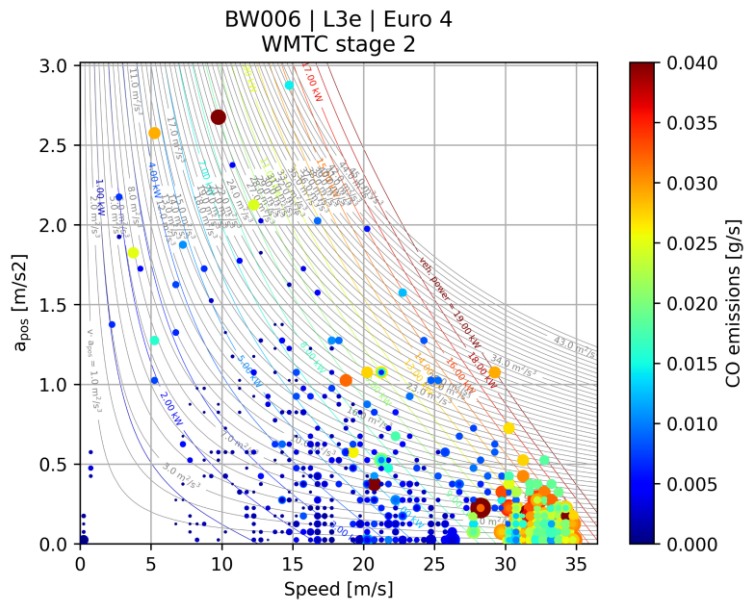
Figure C-14: CO emission map (warm phase)
