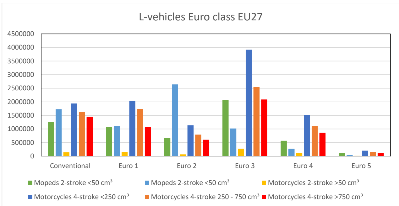
Figure 2-36: Figure 4: Euro class of L-vehicles in the EU27 fleet in 2020. 'Conventional' refer to vehicles without Euro class number, which are from before its introduction
