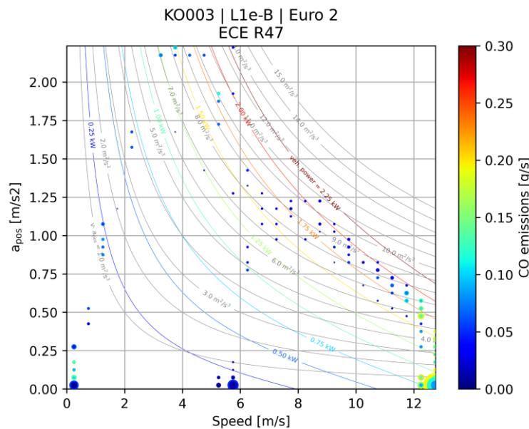
Figure C-2: CO emission map (whole test)
