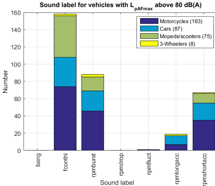
Figure 2-4: Occurrence of events with particular sound labels at 3 locations during 5 days in the Hague, for identified vehicles and near the monitoring positions. fconthi is the same as rpbmconthi
