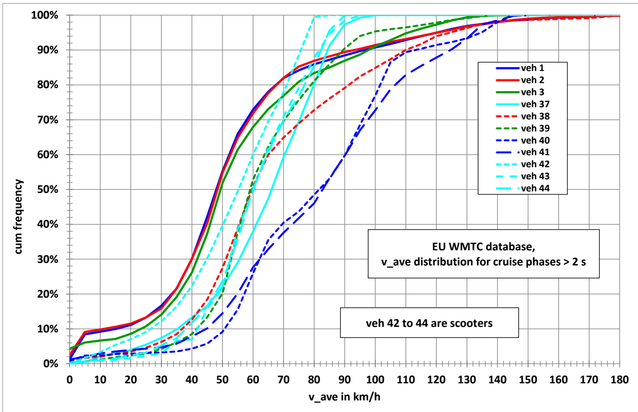
Figure 2-25: v_{ave} frequency distributions for cruise phases > 2 s
