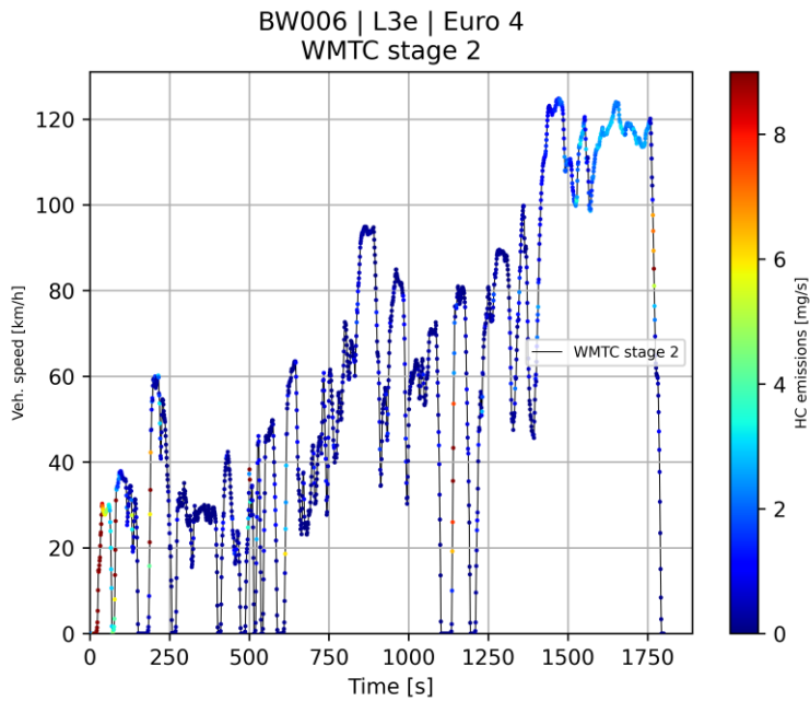
Figure C-16: Overview of HC emissions
