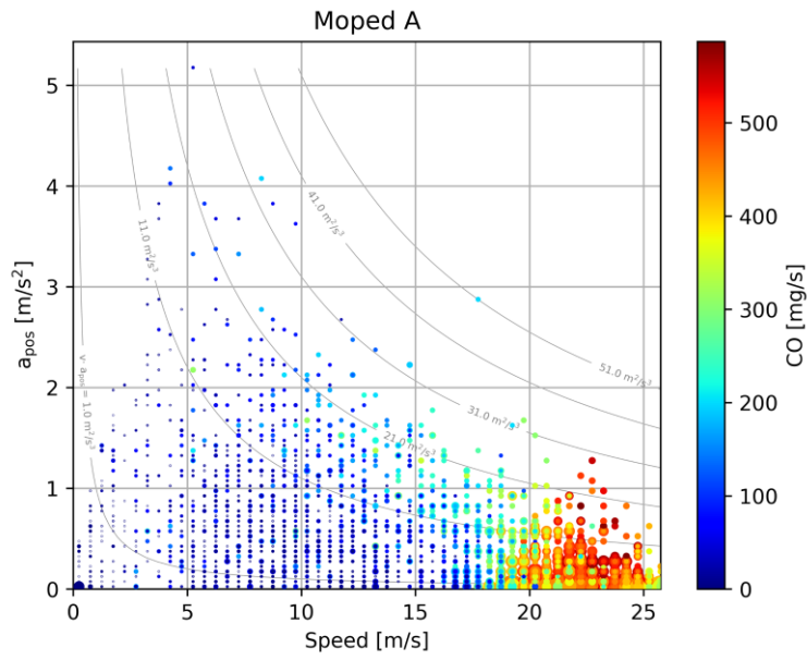
Figure C-22: CO emissions of moped A
