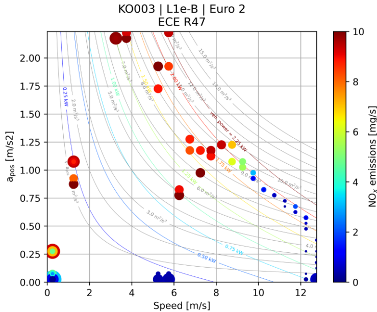
Figure 2-18: NO x emission map of a moped on the UN ECE R47 cycle (warm start phase)
