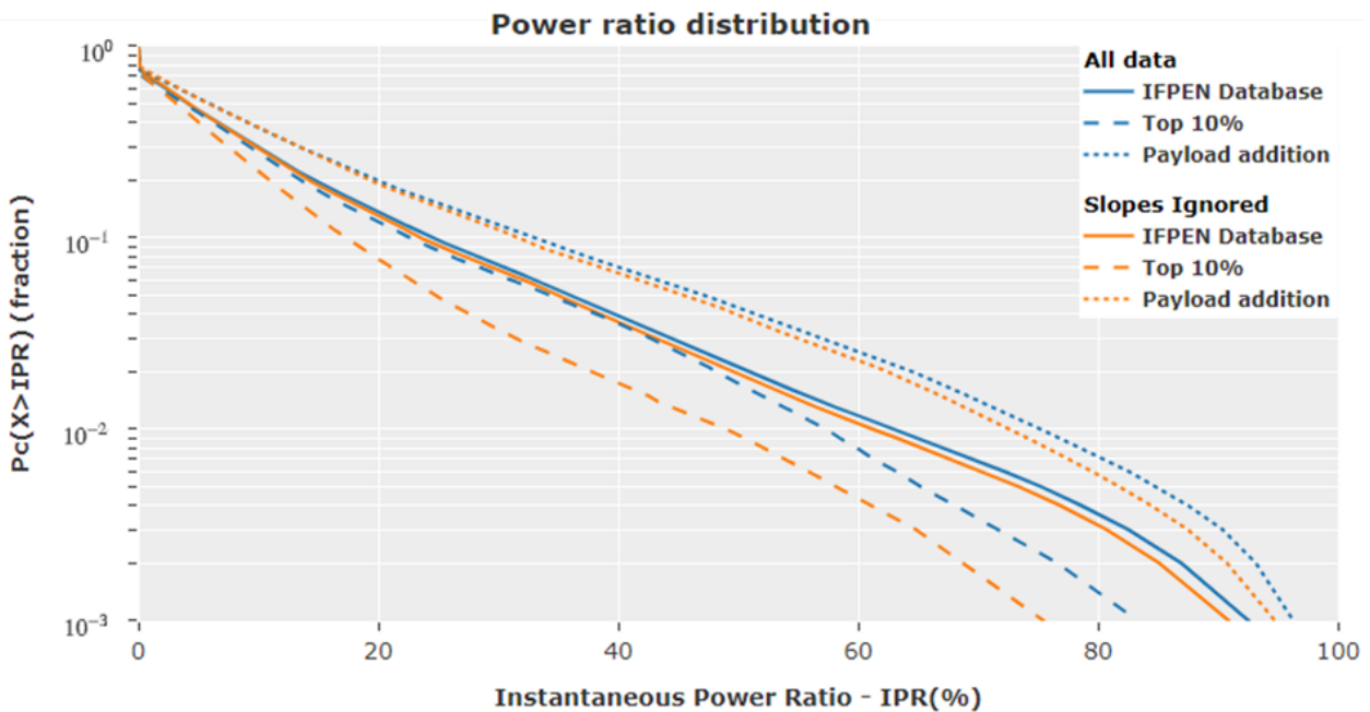
Figure 2-14: Instantaneous power ratio probability distribution
