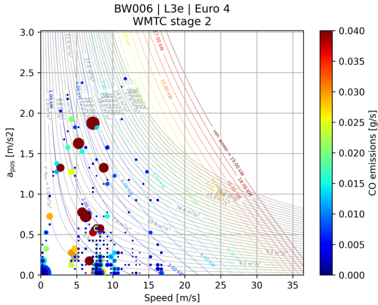
Figure C-13: CO emission map (cold phase)
