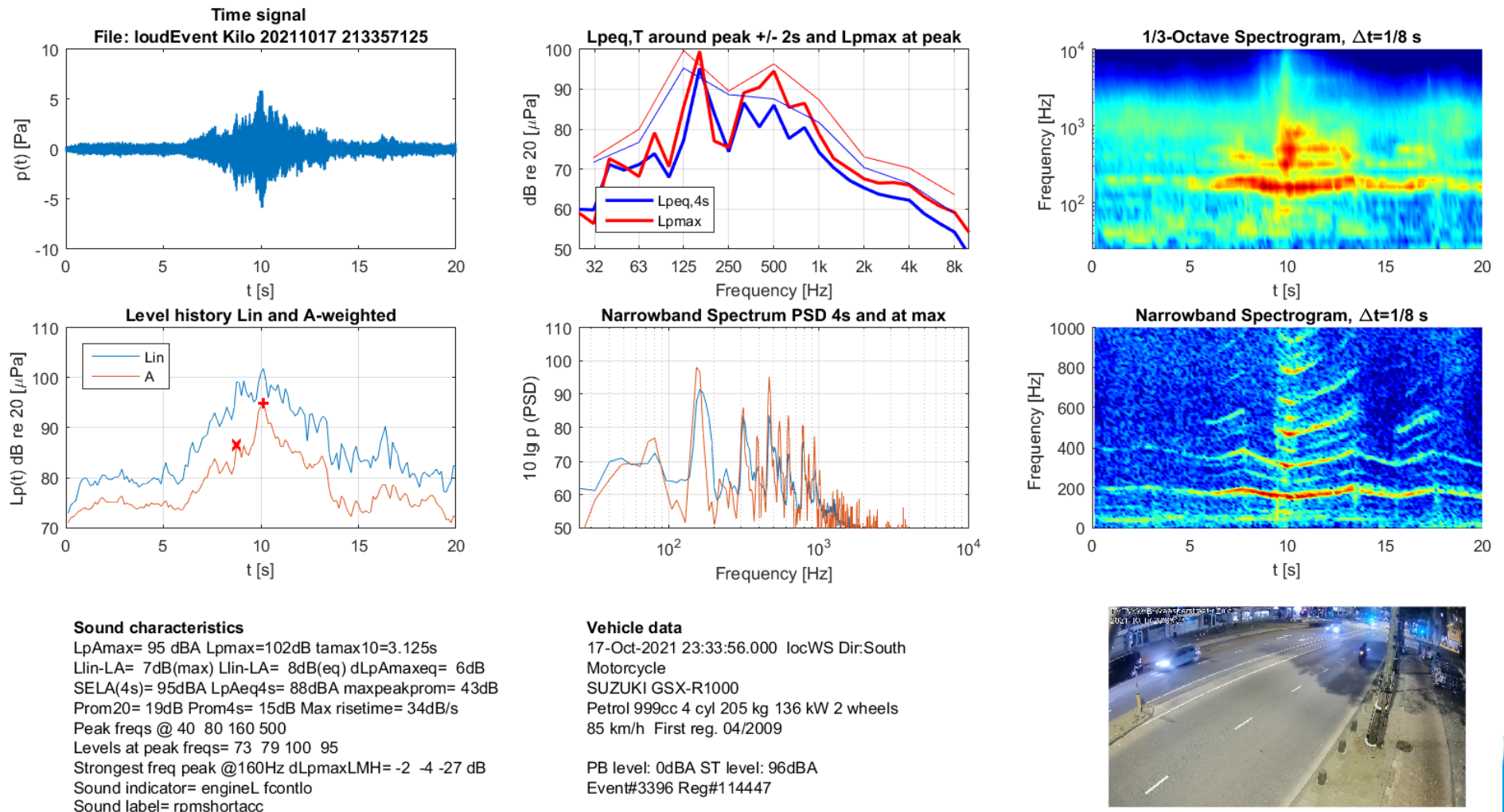
Figure B-6: Sound characteristics of a motorcycle, example of 'rpmshortacc'
