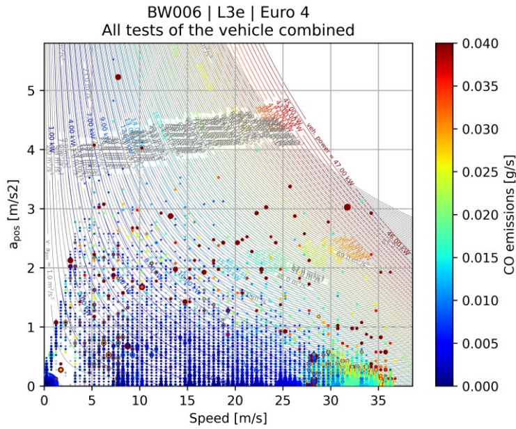
Figure C-15: CO emission map (all tests combined)
