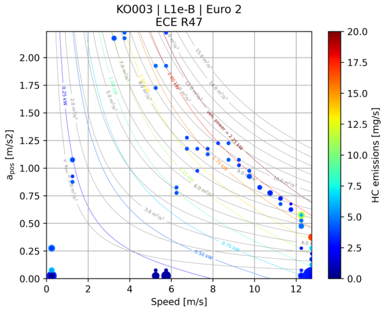
Figure C-9: HC emission map (warm phase)
