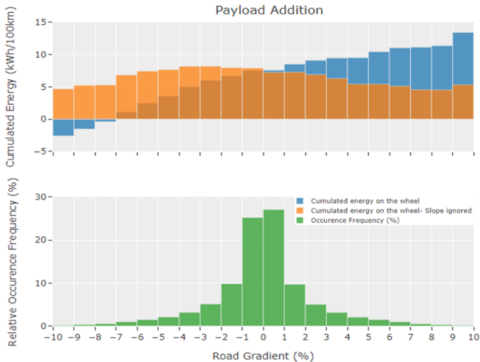
Figure 2-13: Specific cumulative energy on the wheel binned by road gradient and relative occurrence frequency of each road gradient bin – Payload addition (second passenger)
