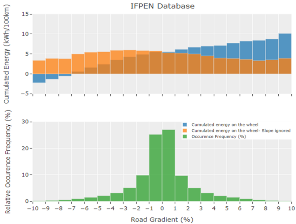
Figure 2-11: Specific cumulative energy on the wheel binned by road gradient and relative occurrence frequency of each road gradient bin – IFPEN Database
