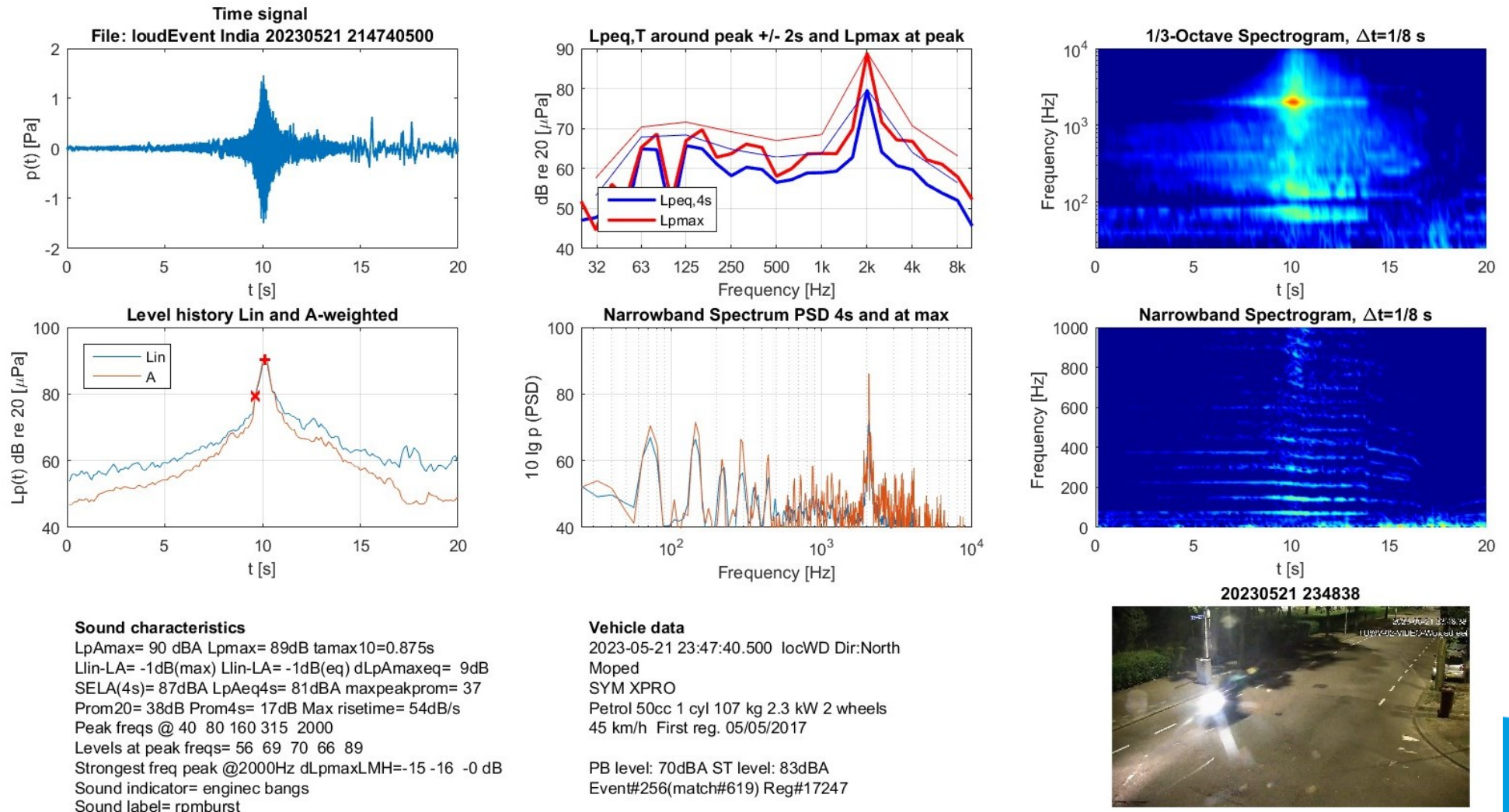
Figure B-16: Sound characteristics of a moped, example of 'rpmburst'
