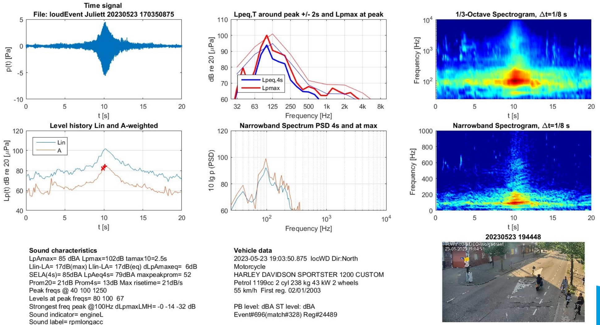
Figure B-24: Sound characteristics of a motorcycle, example of 'rpmlongacc'
