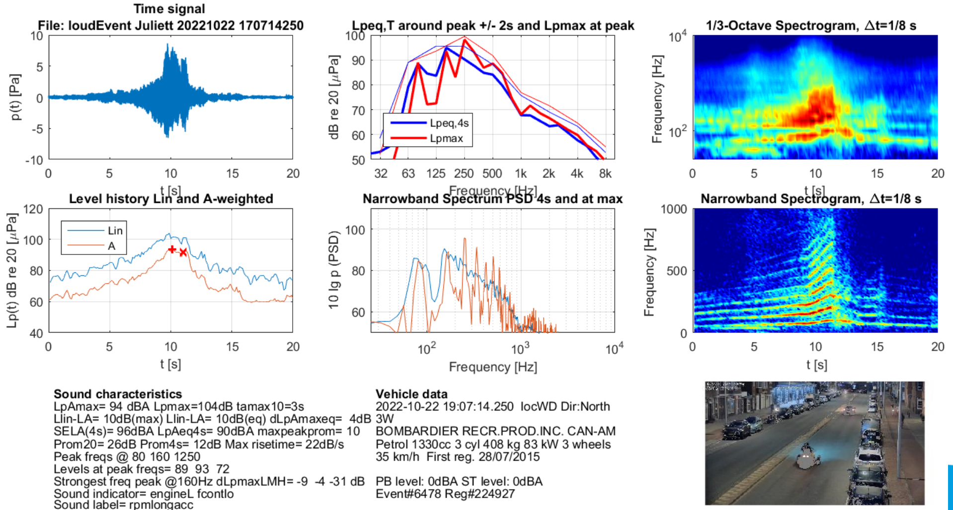
Figure B-12: Sound characteristics of a trike, example of 'rpmlongacc'
