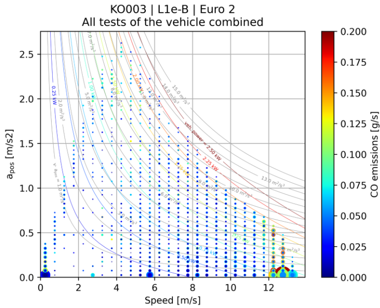
Figure C-5: CO emission map (all tests combined)
