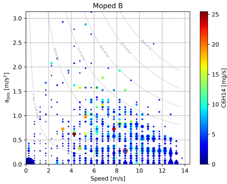
Figure C-26: HC emissions of moped B
