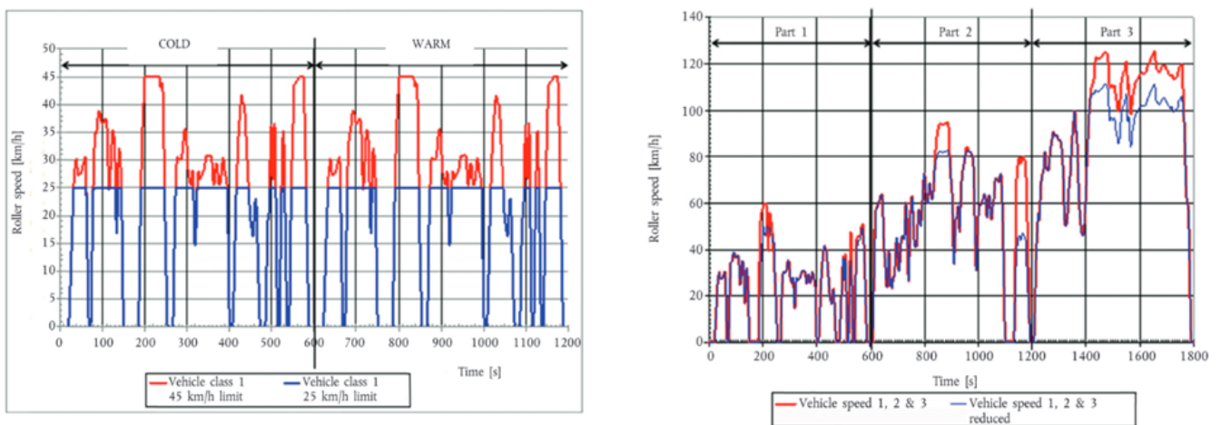
Figure 3-9: Vehicle speed time series of the WMTC cycle (left figure is for class 1 vehicles only)
