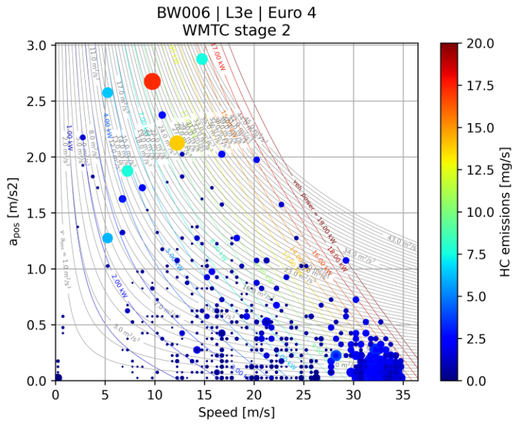
Figure C-19: HC emission map (warm phase)
