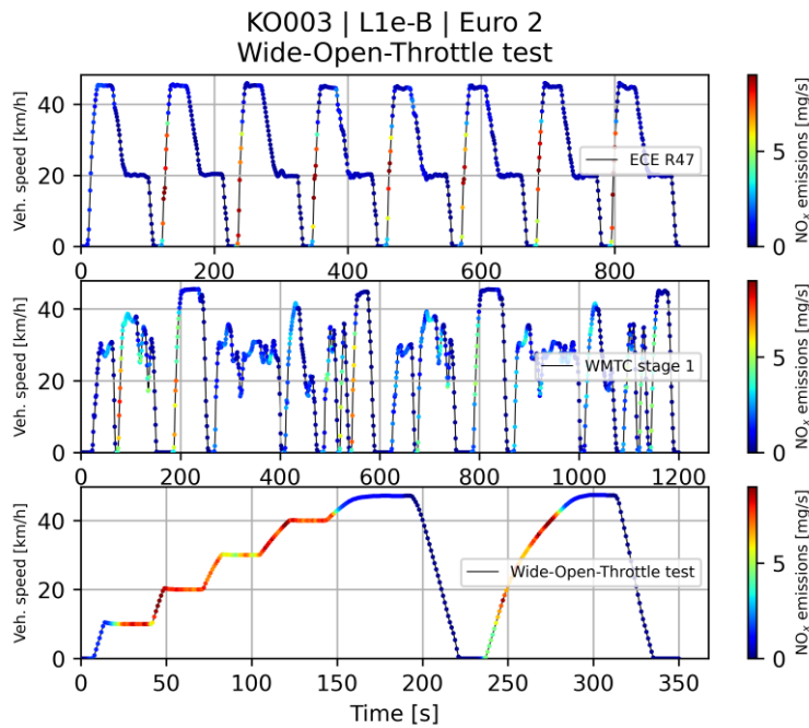
Figure 2-15: Instantaneous NO x mass emission of different tests
