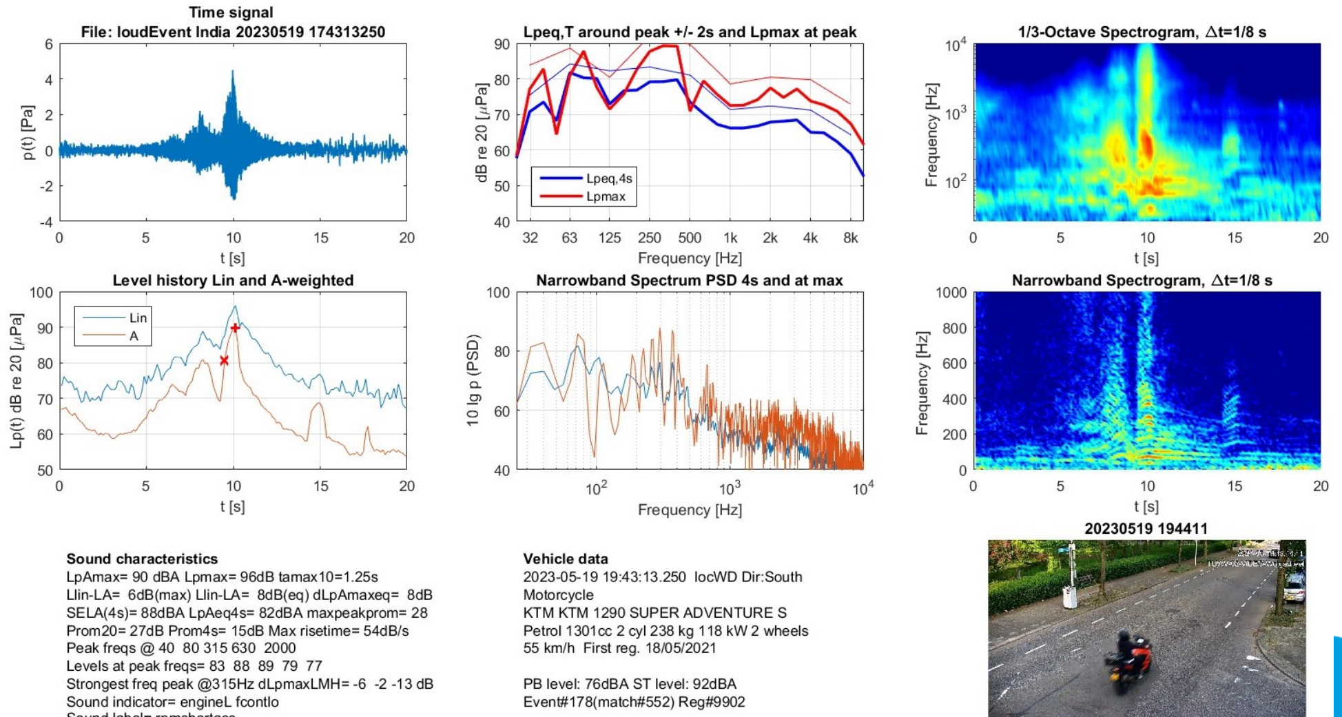
Figure B-15: Sound characteristics of a motorcycle, example of 'rpmshortacc'
