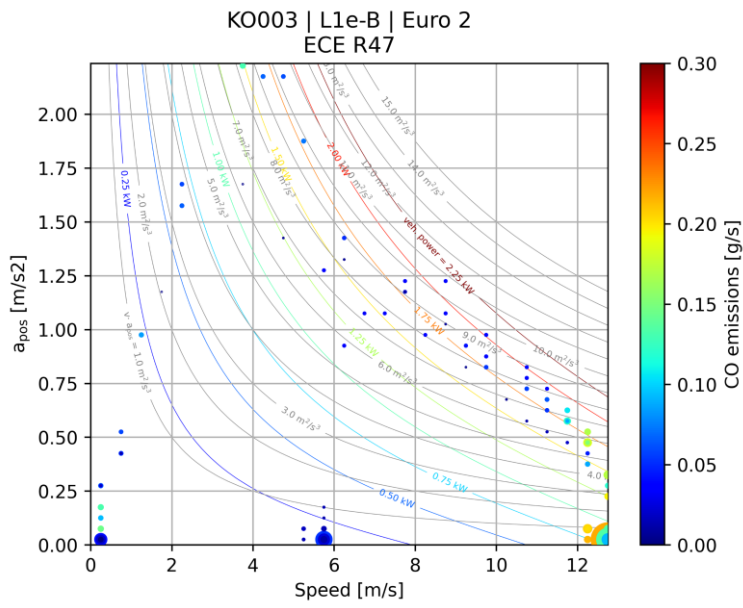
Figure C-3: CO emission map (cold phase)
