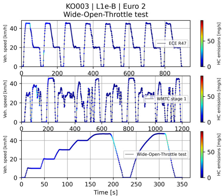
Figure C-6: Overview of HC emissions of different test cycles
