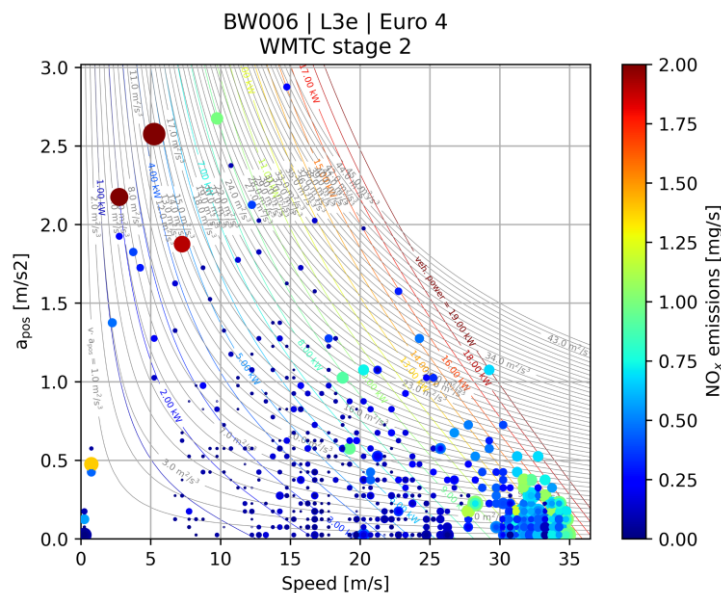
Figure 2-23: NO x emission map of a motorcycle on the WMTC Stage 2 cycle (warm phase)
