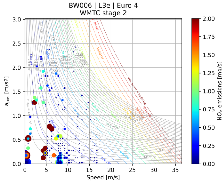
Figure 2-22: NO x emission map of a motorcycle on the WMTC Stage 2 cycle (cold start phase)
