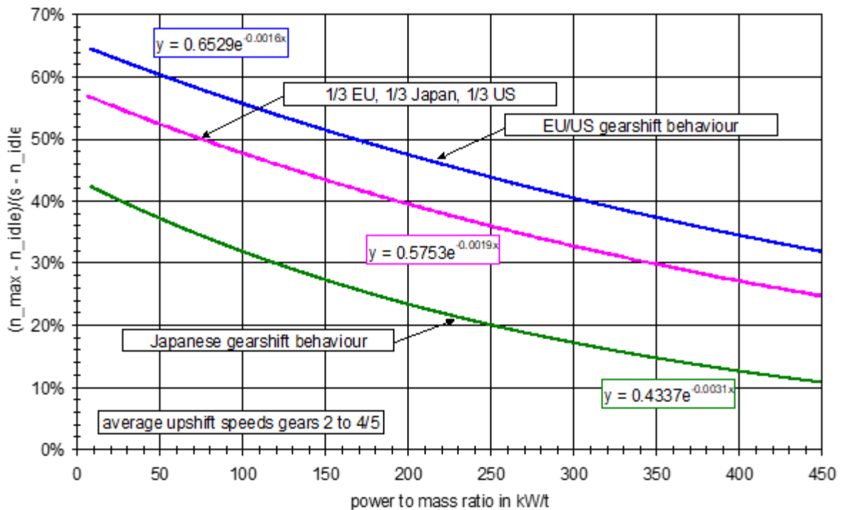
Figure 3-4: The final approximation function for upshift speeds in gears higher than 1 (1/3 Europe, 1/3 Japan, 1/3 USA). From ECE/TRANS/180/Add.2/Appendix 1 (Technical Report to GTR 2), s means rated engine speed
