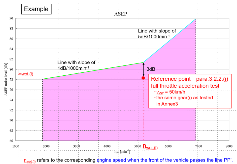
Figure 3-3: Example of ASEP test range showing the ASEP sound limit line based on the reference point from the normal WOT test. Any points measured for ASEP must be below the limit line. Taken from IMMA presentation at GRB ASEP meeting 11-13 July 2017 [12].
