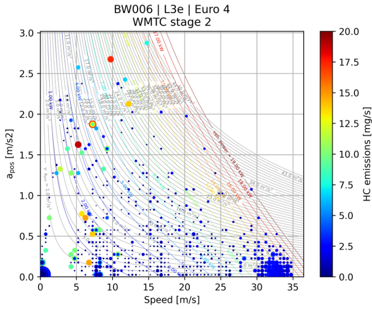
Figure C-17: HC emission map (whole test)
