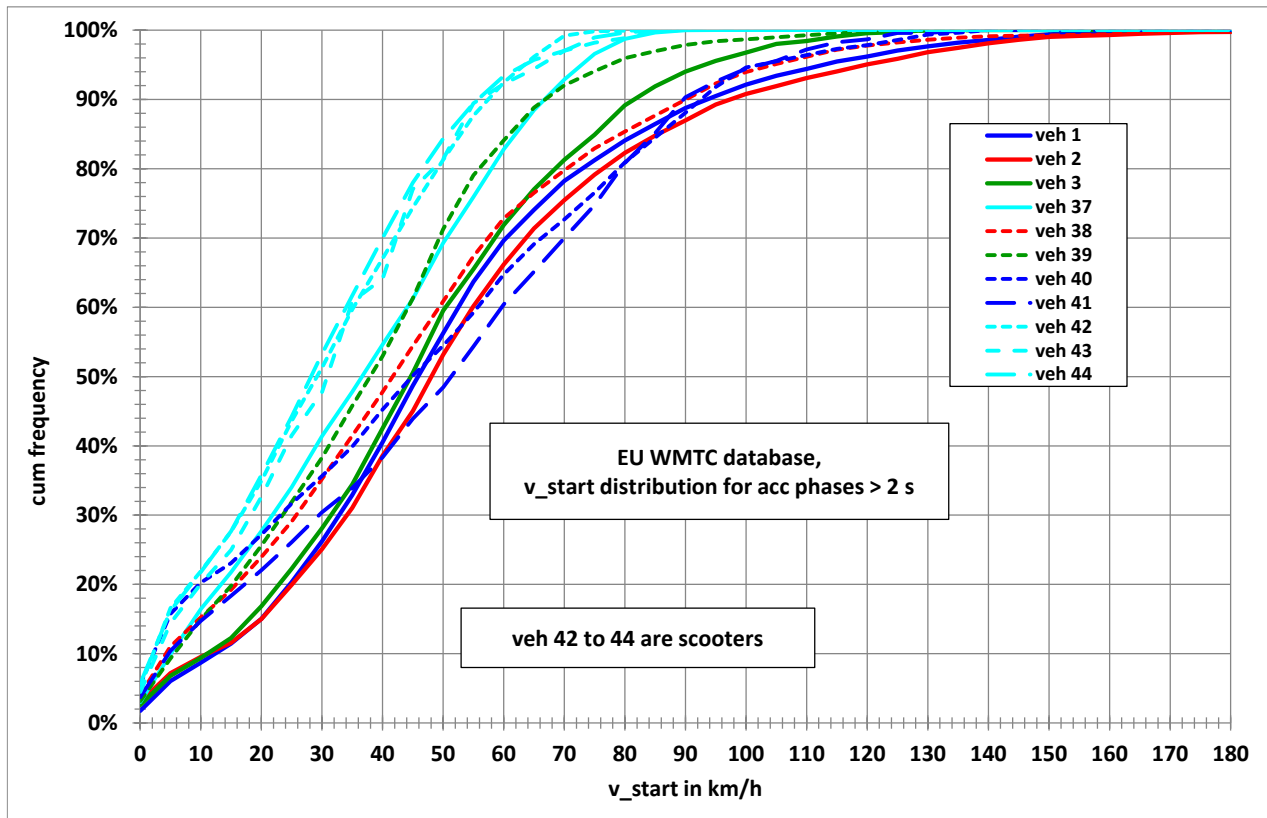
Figure 2-24: v_{start} frequency distributions for acc phases > 2 s
