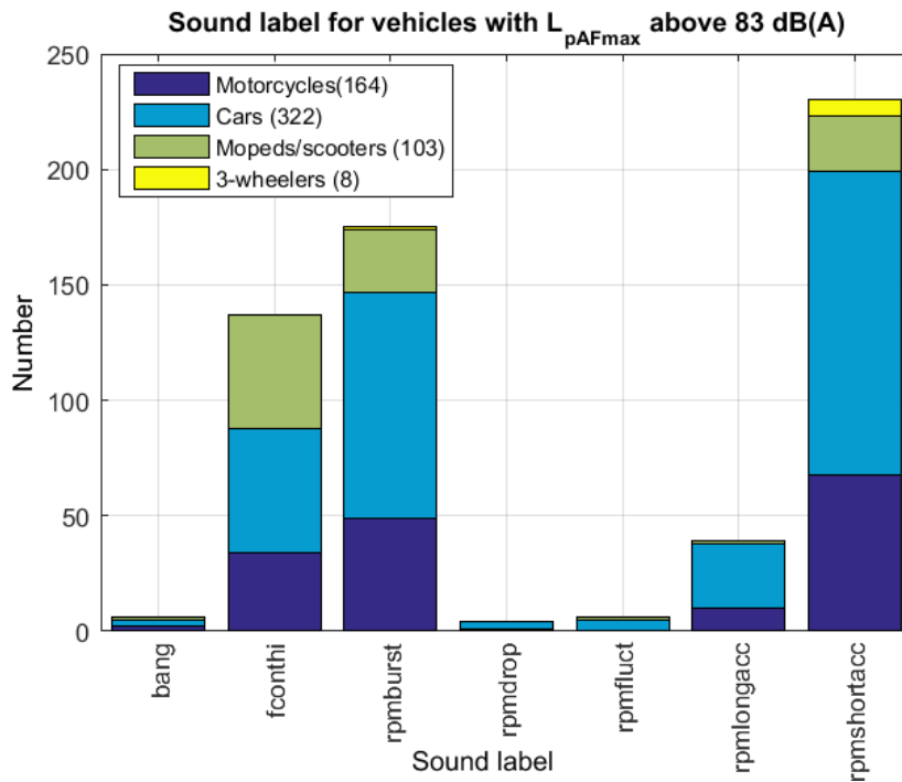
Figure 2-3: Occurrence of events with particular sound labels at 3 locations during 5/10 days in Rotterdam, for identified vehicles and near the monitoring positions. fconthi is the same as rpbmconthi
