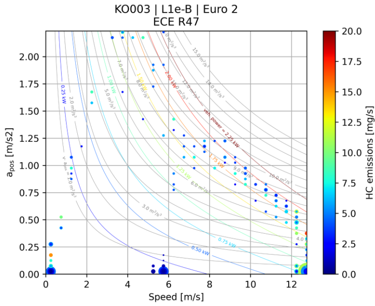
Figure C-7: HC emission map (whole test)
