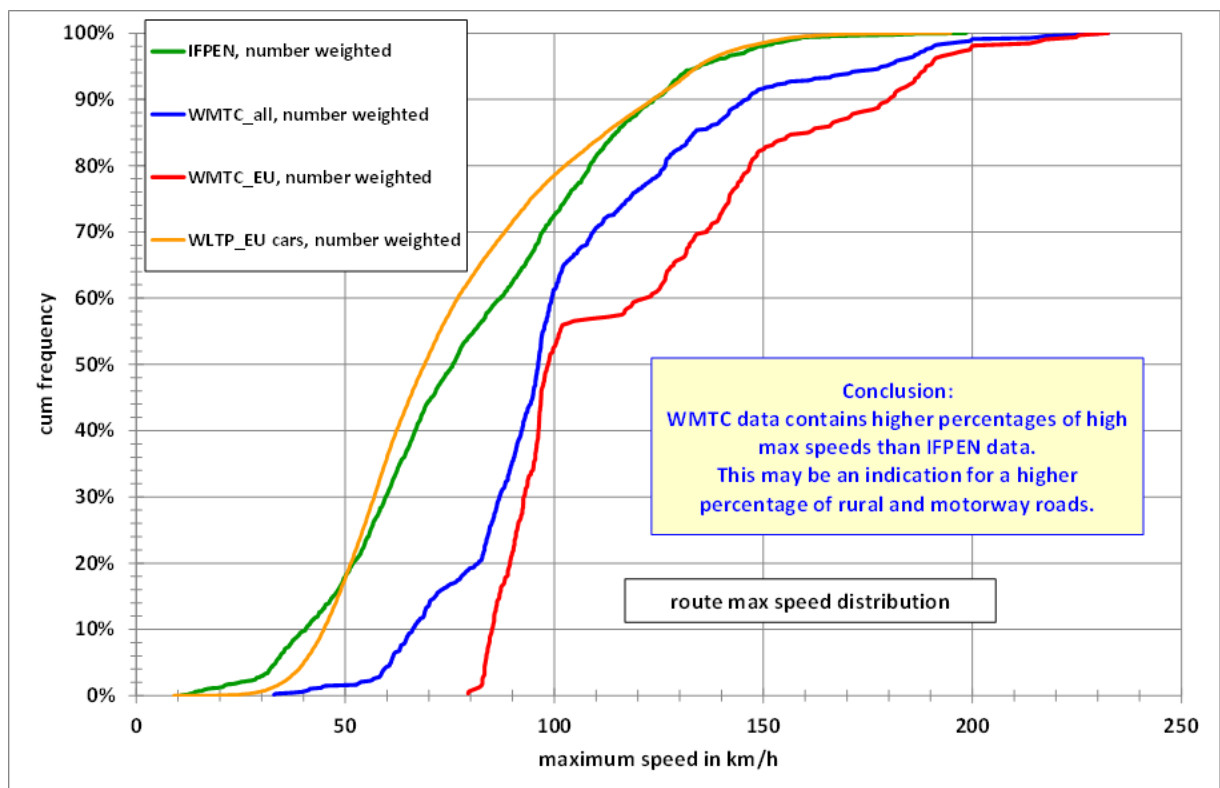
Figure 2-7: Distributions of maximum speed values per trip
