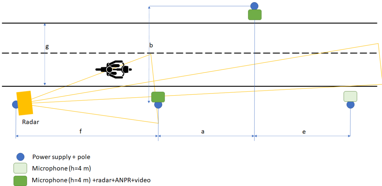
Figure 2-27: Measurement configuration. The dimensions a-g are different for each site, listed in Annex B.
