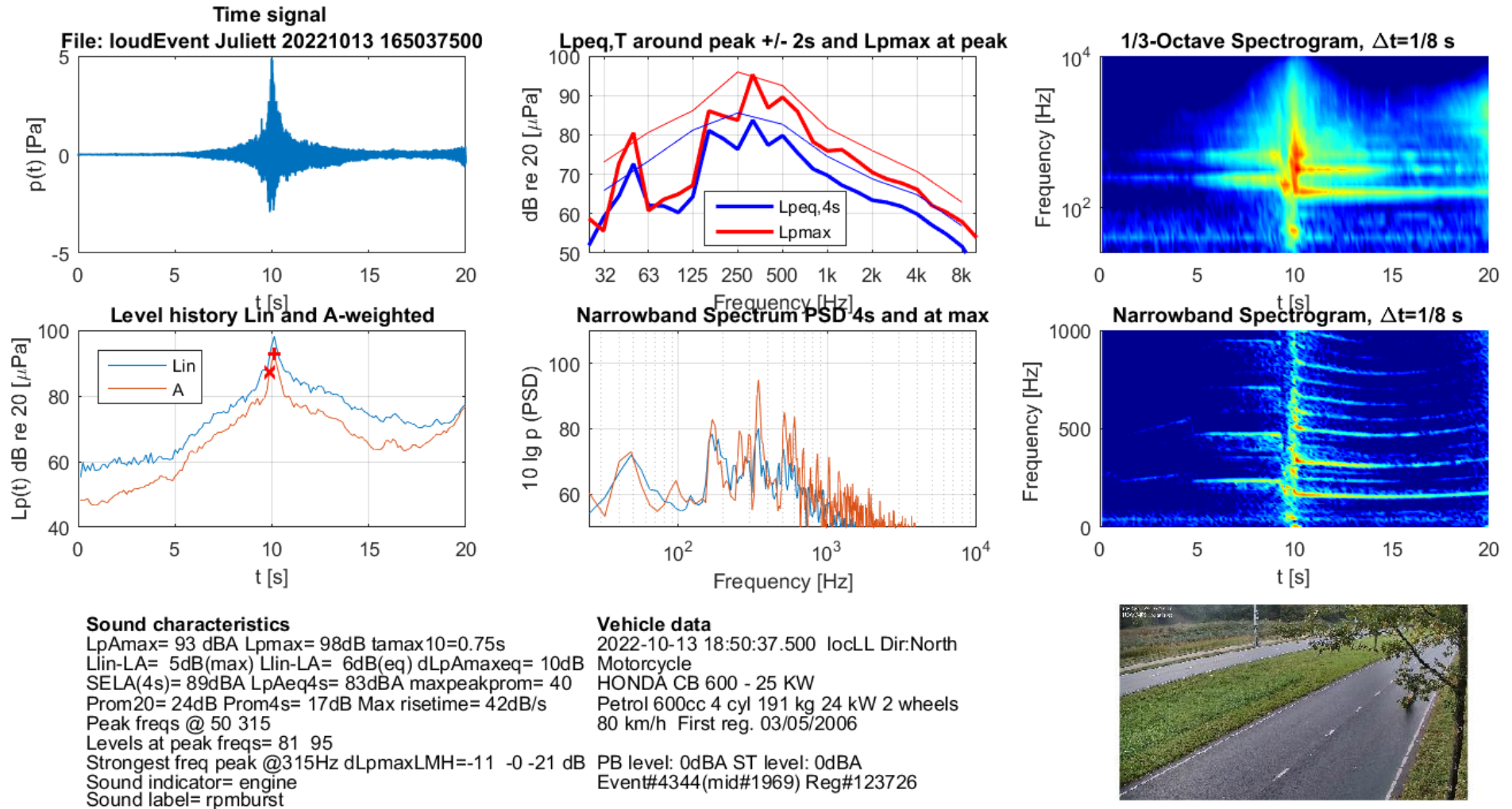
Figure B-10: Sound characteristics of a motorcycle, example of 'rpmburst' due to high speed and close range
