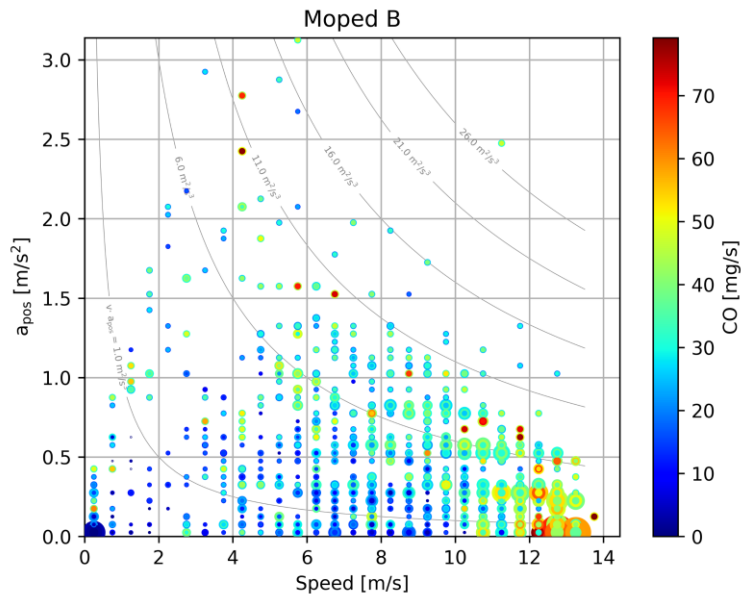
Figure C-25: CO emissions of moped B
