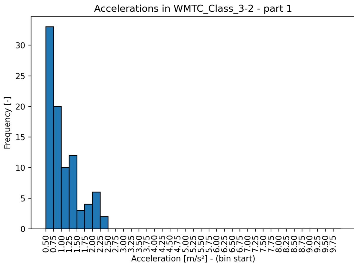
Figure 2-32: Maximum acceleration distribution for WMTC part I (urban part)
