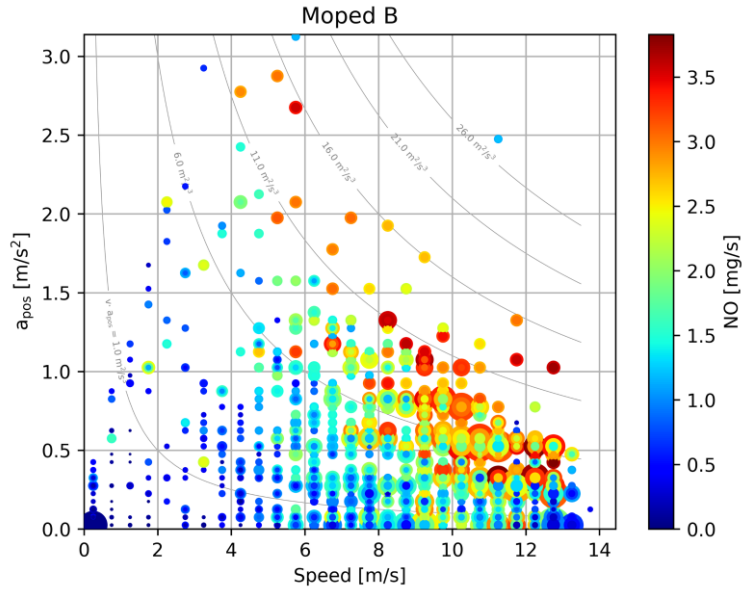
Figure C-24: NO emissions of moped B
