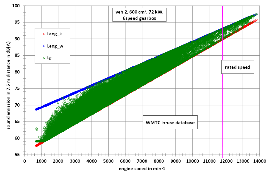
Figure 2-2: Noise emission of a sports bike in dependence of engine speed and vehicle speed modelled for in-use data of the WMTC database. (Leng_k – noise emission at low or no load condition, Leng_w – noise emission at wide open throttle or full load condition, Lg – second by second noise emission for the in-use data)
