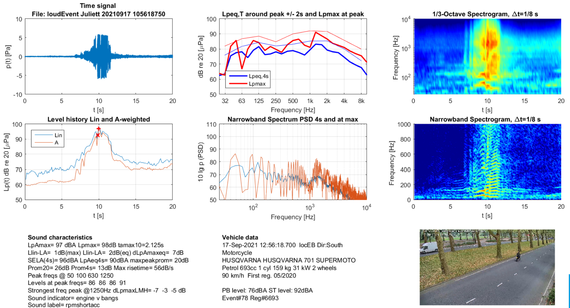
Figure B-7: Sound characteristics of a motorcycle, example of 'rpmsshortacc'
