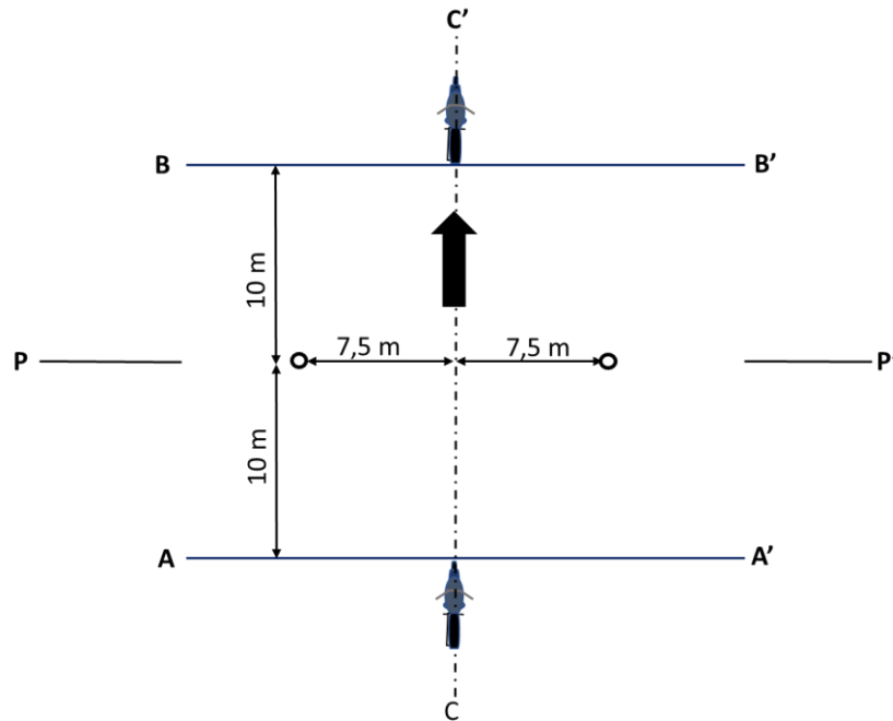
Figure 3-1: Test setup for pass-by sound measurement for L-vehicles. The vehicle approaches AA' and proceeds with wide open throttle, which is released at BB'.
