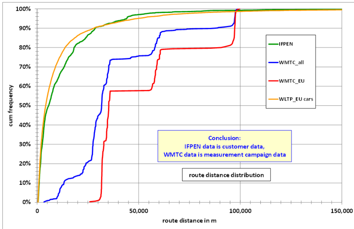
Figure 2-5: Trip or route distance distributions for the different L-category vehicles datasets
