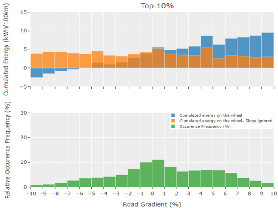
Figure 2-12: Specific cumulative energy on the wheel binned by road gradient and relative occurrence frequency of each road gradient bin – Top 10% most severe trips in terms of ascending slope
