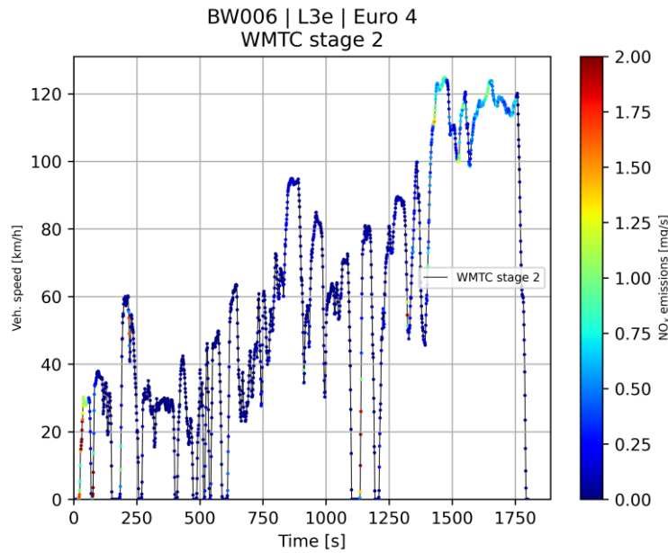
Figure 2-20: Instantaneous NO x mass emission of the WMTC Stage 2 test
