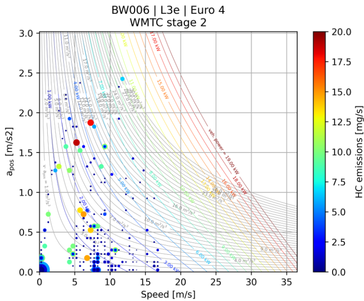
Figure C-18: HC emission map (cold phase)
