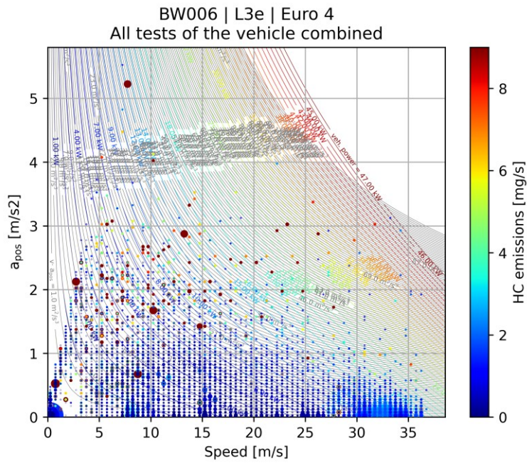
Figure C-20: HC emission map (all tests combined)
