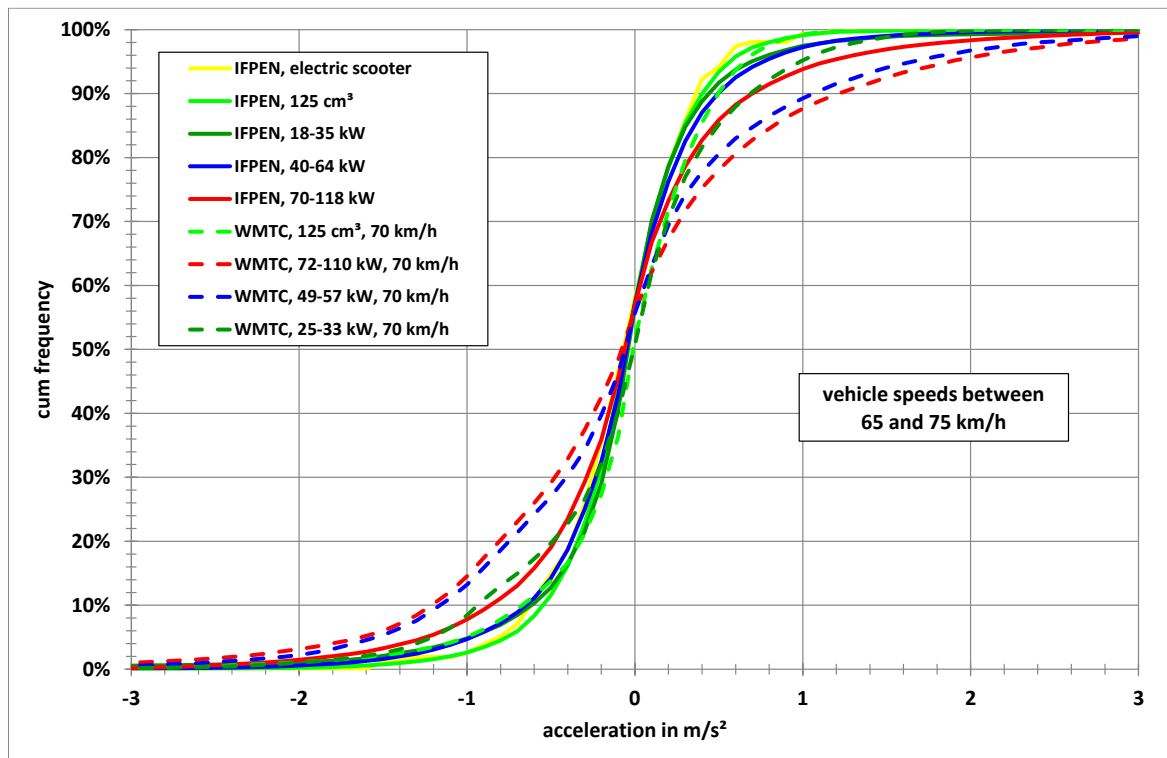
Figure 2-10: Distributions of acceleration values at vehicle speeds around 70 km/h for the different vehicle classes as specified above
