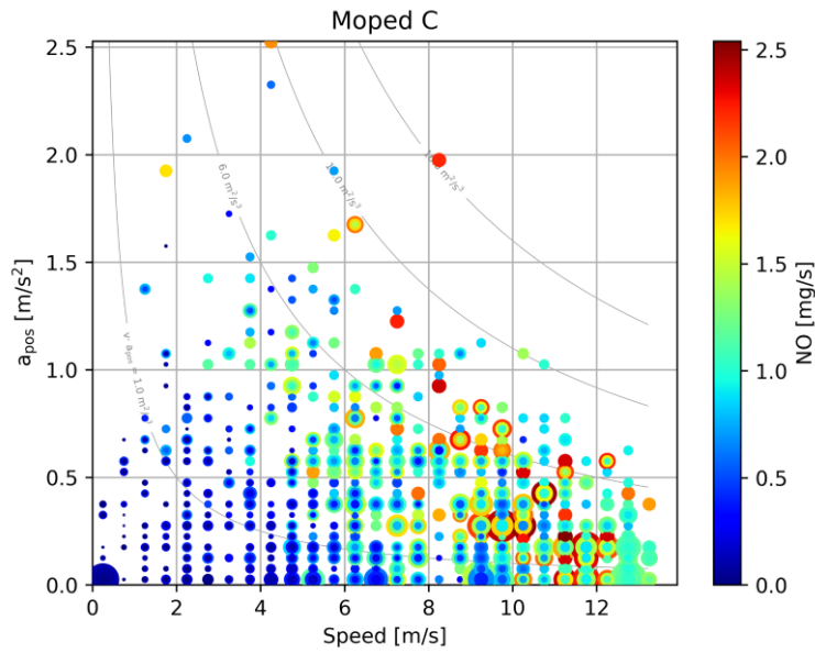
Figure C-27: NO emissions of moped C
