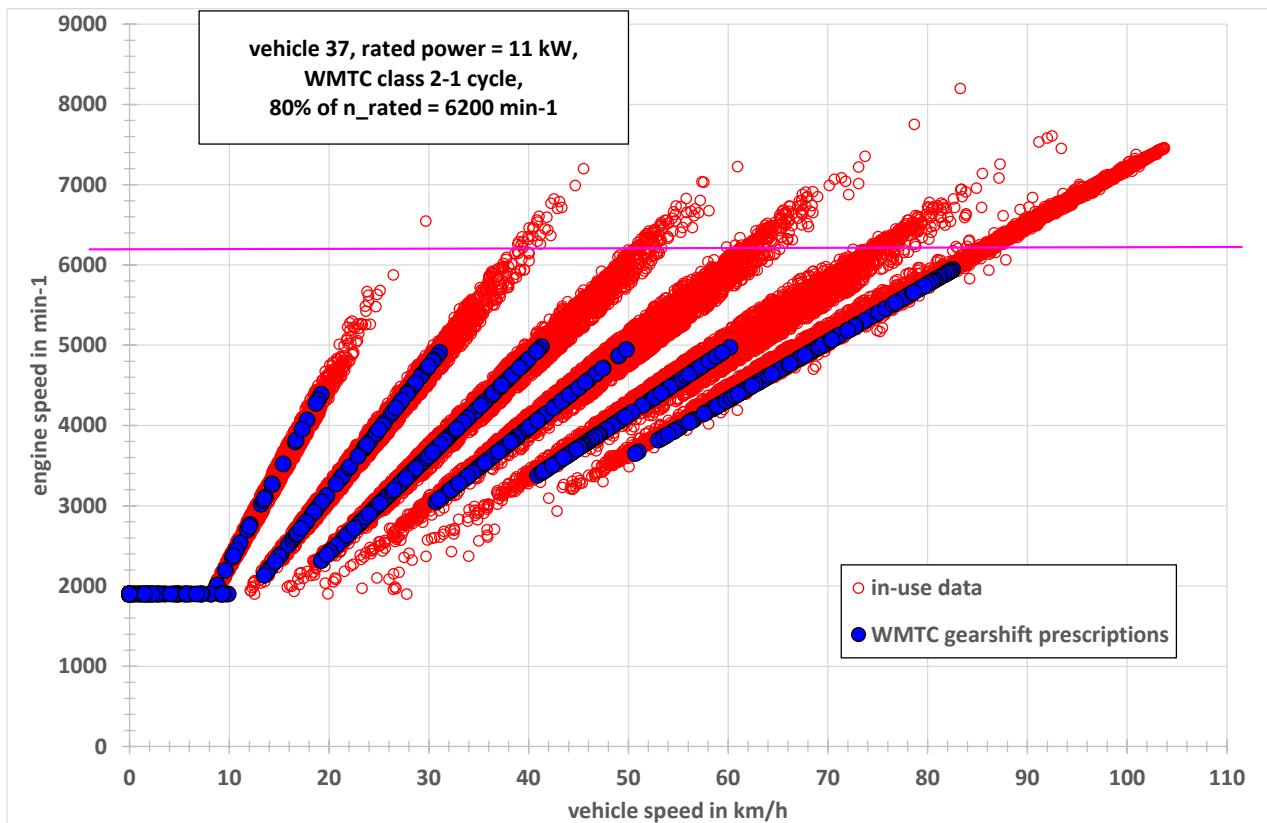
Figure 3-8: Engine speed versus vehicle speed plots for the WMTC cycle and WMTC in-use data for vehicle 37
