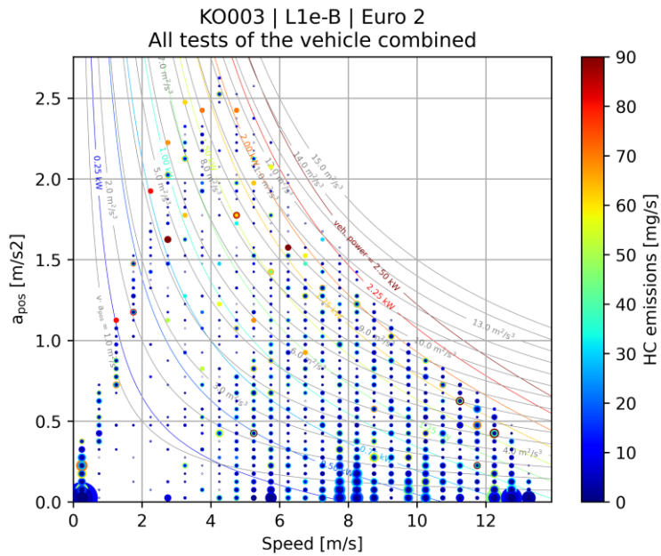
Figure C-10: HC emission map (all tests combined)
