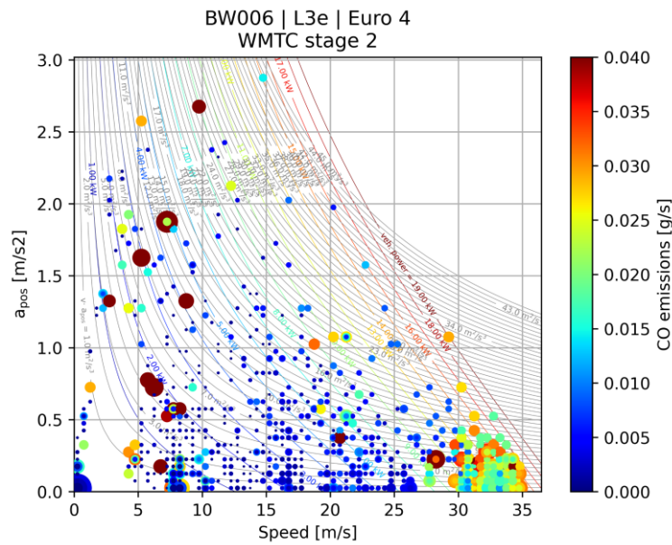
Figure C-12: CO emission map (whole test)
