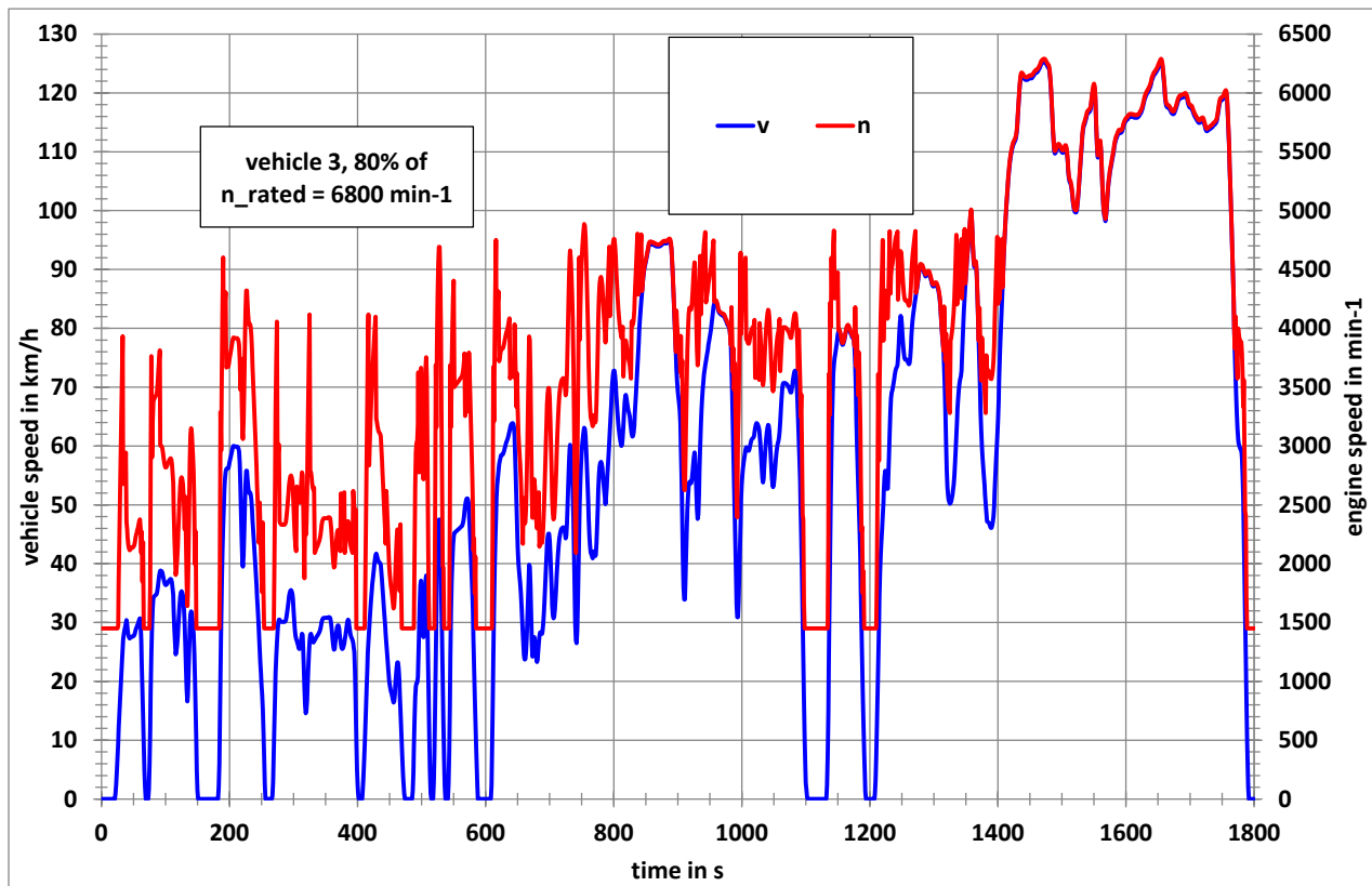
Figure 3-5: Vehicle and engine speed time series of the WMTC cycle for vehicle 3 of the EU WMTC in use database
