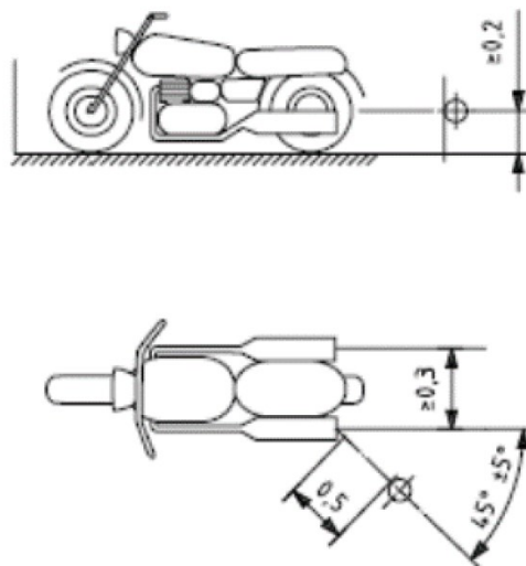
Figure 3-2: Test setup for stationary sound measurement of L-vehicles for roadside checks. The engine runs at constant specified speed, and the throttle is released.
