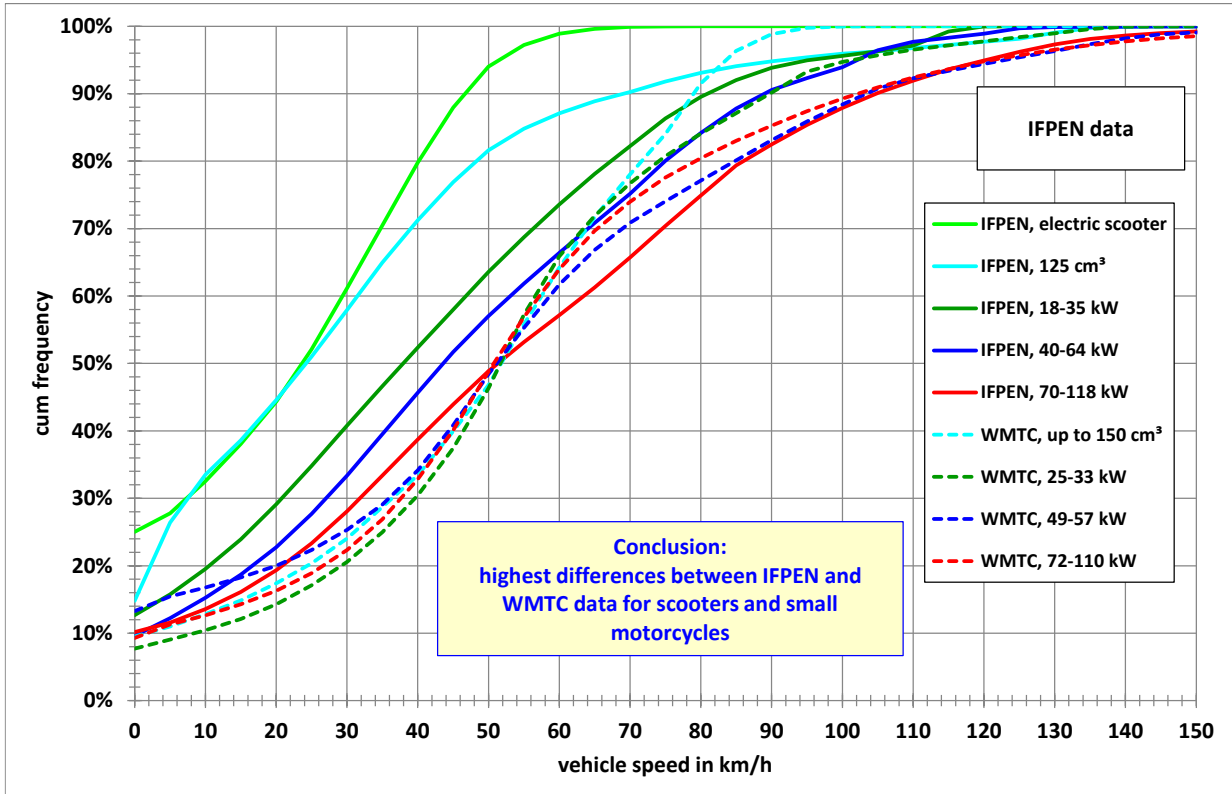
Figure 2-8: Distributions of vehicle speeds for the different vehicle classes as specified above
