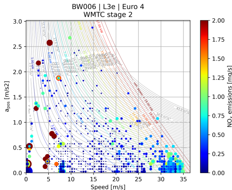
Figure 2-21: NO x emission map of a motorcycle on the WMTC Stage 2 cycle
