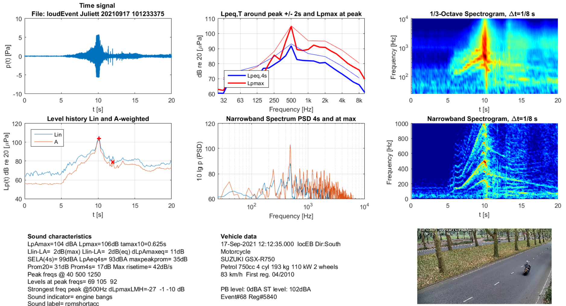
Figure B-5: Sound characteristics of a motorcycle, example of 'rpmshortacc'
