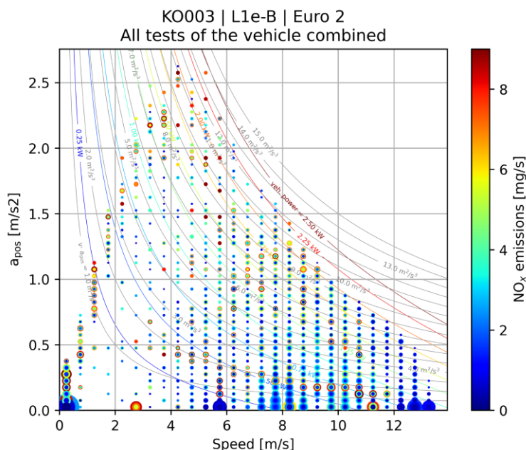
Figure 2-19: Combined NO x emission map of a moped
