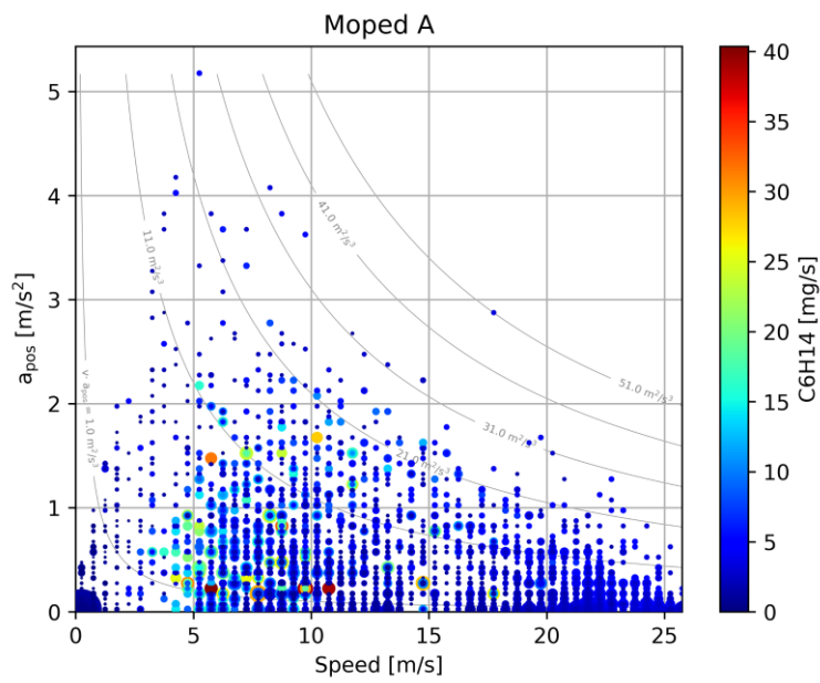
Figure C-23: HC emissions of moped A
