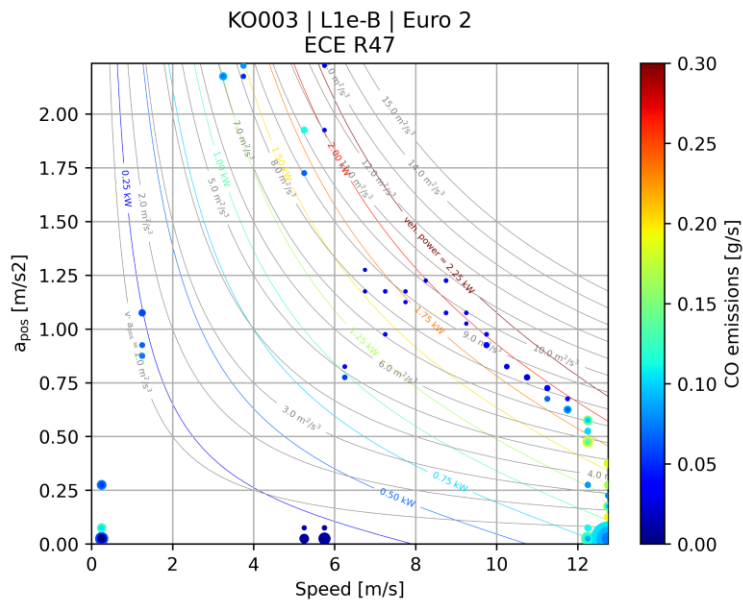
Figure C-4: CO emission map (warm phase)
