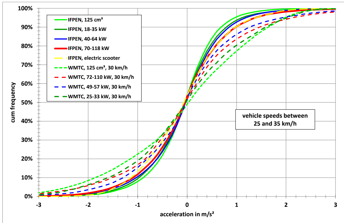
Figure 2-9: Distributions of acceleration values at vehicle speeds around 30 km/h for the different vehicle classes as specified above
