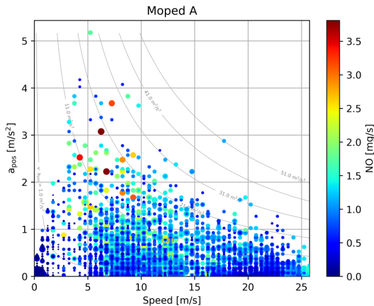
Figure C-21: NO emissions of moped A
