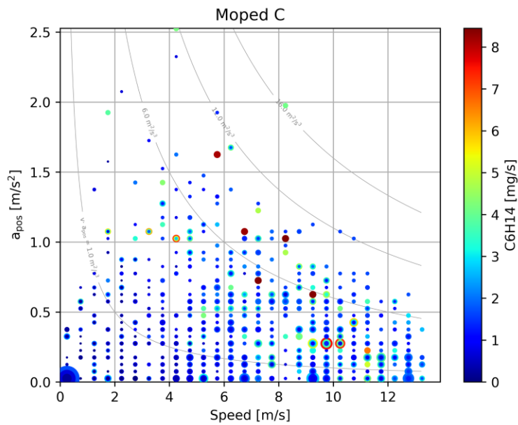
Figure C-29: HC emissions of moped C
