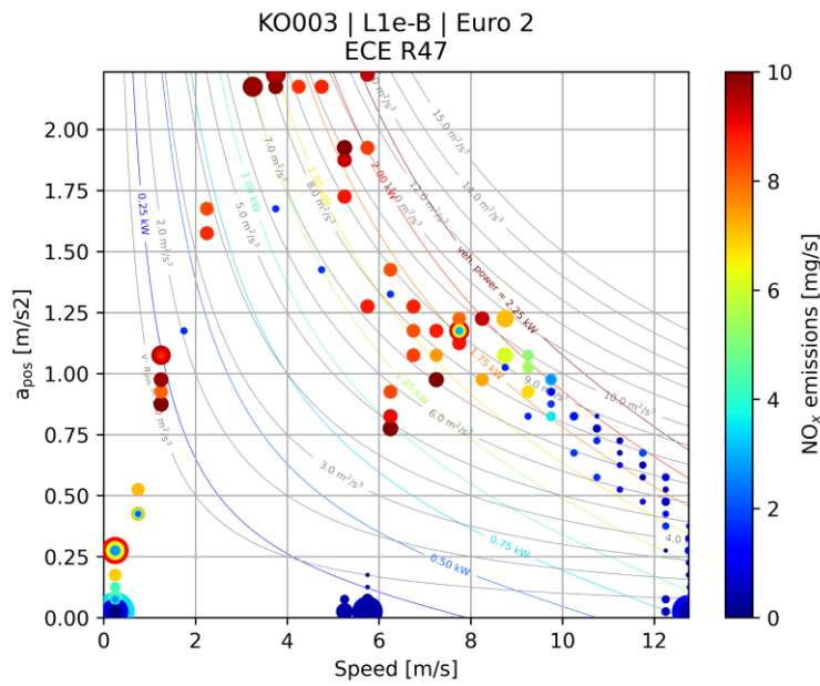
Figure 2-16: NO x emission map of a moped on the UN ECE R47 cycle
