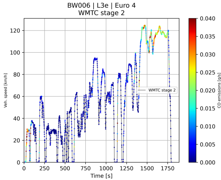
Figure C-11: Overview of CO emissions
