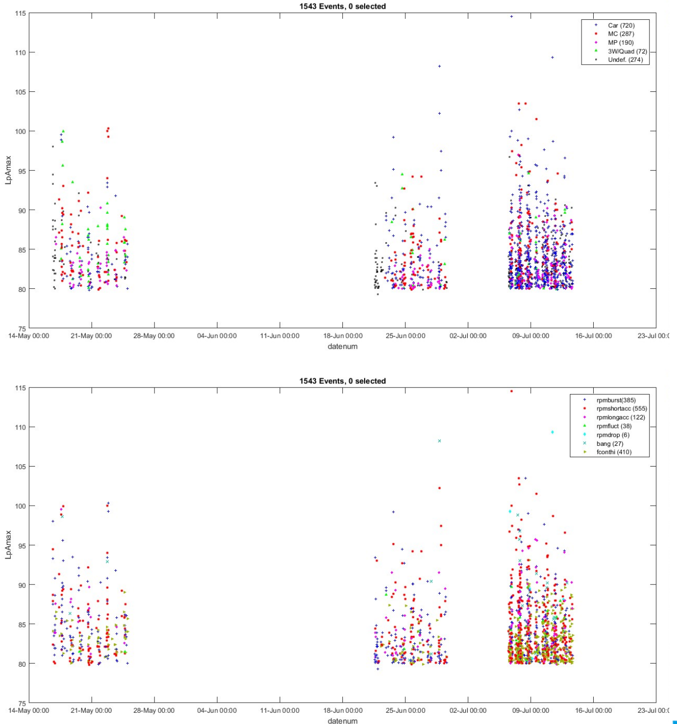
Figure 2-30: Vehicle pass-by sound levels L_{pA_{max}} above 80 dB(A) for three locations measured at two roadside positions. Top: showing vehicle type where identified; bottom: same data but indicating the vehicle sound label.
