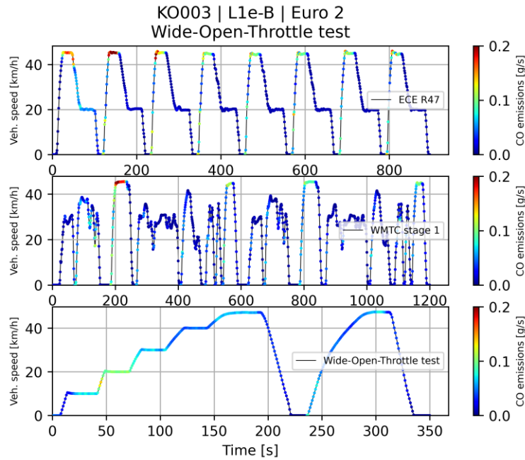
Figure C-1: Overview of CO emissions of different test cycles
