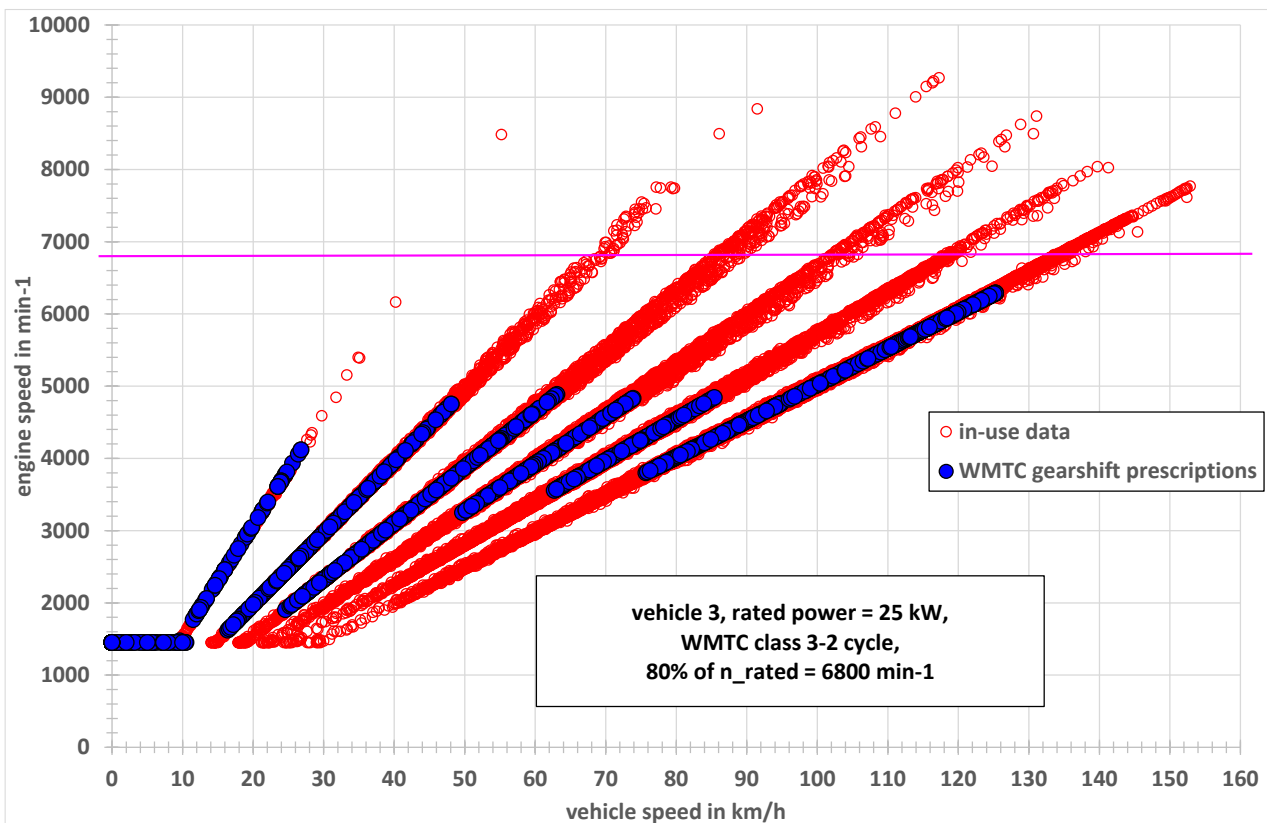
Figure 3-6: Engine speed versus vehicle speed plots for the WMTC cycle and WMTC in-use data for vehicle 3
