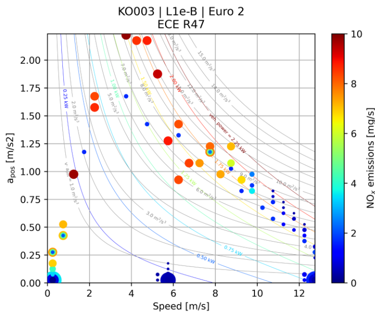
Figure 2-17: NO x emission map of a moped on the UN ECE R47 cycle (cold start phase)
