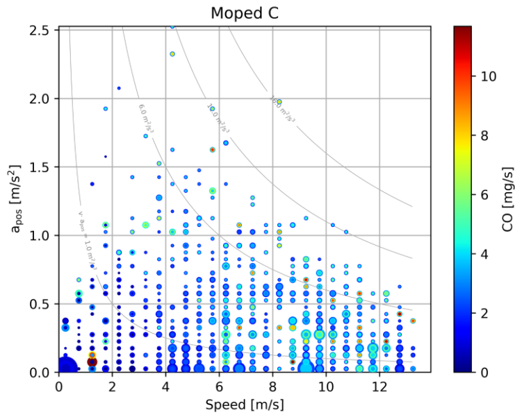
Figure C-28: CO emissions of moped C
